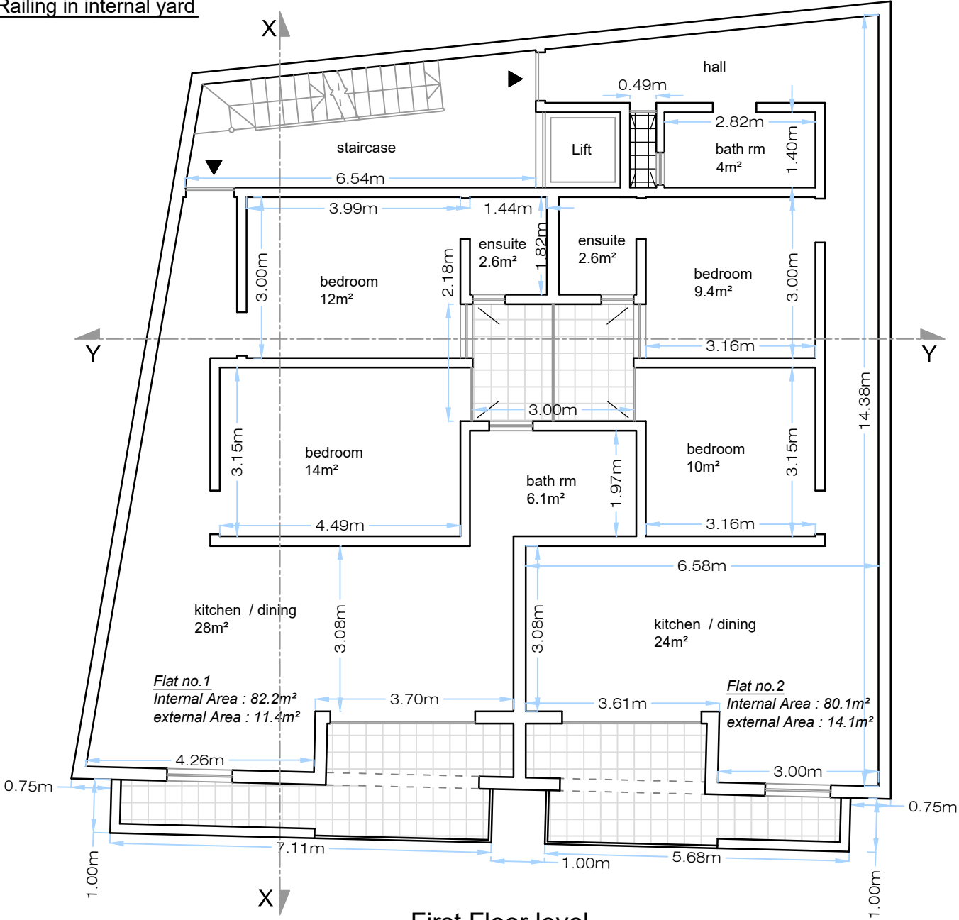
First Floor level proposed scale 1 : 100
