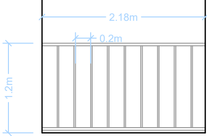
Detail of Railing in internal yard Scale 1:50
